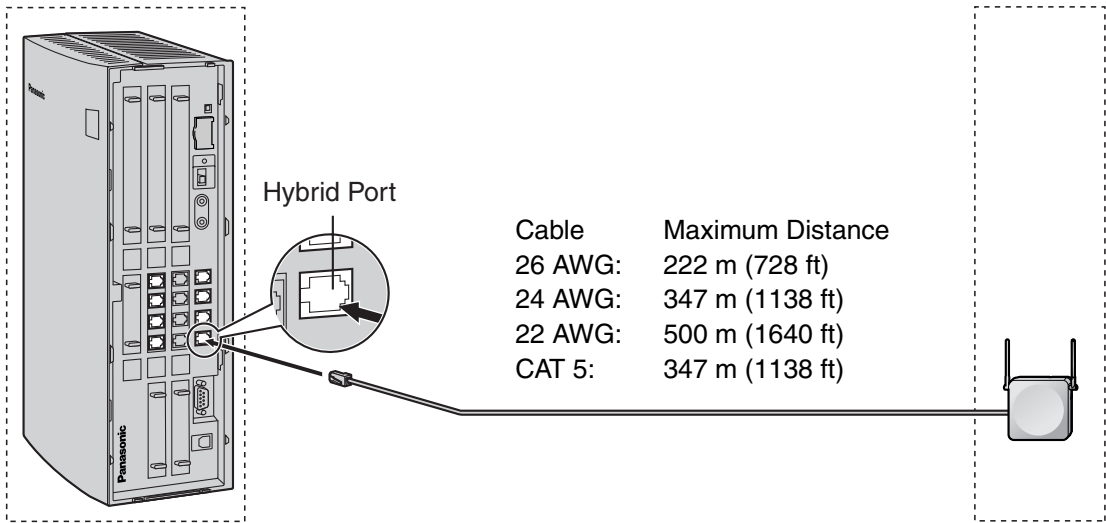
A Hybrid Port or HLC4 card (RJ11)
